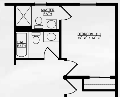
OPT. MASTER BATH
