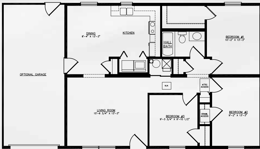
CRAWLSPACE PLAN
